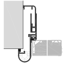
EUROFI-E Eckzarge
